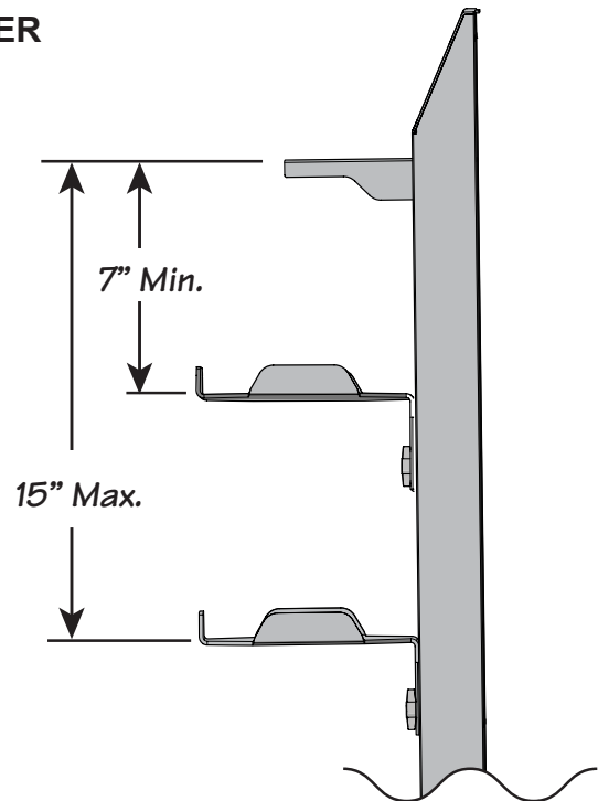
Variable Height Adjustment The StaySafe Can Accommodate Bottles of Most Shapes and Size
