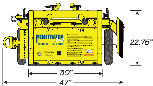
Larger Fall Arrest Rings are Side By Side. Provides industry leading security connection points.
